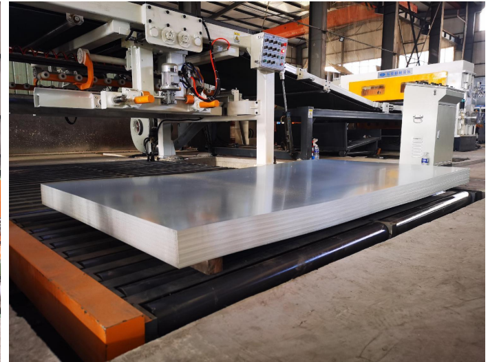
Cross cutting flying shear equipment, high efficiency, cost reduction and efficiency increase.
