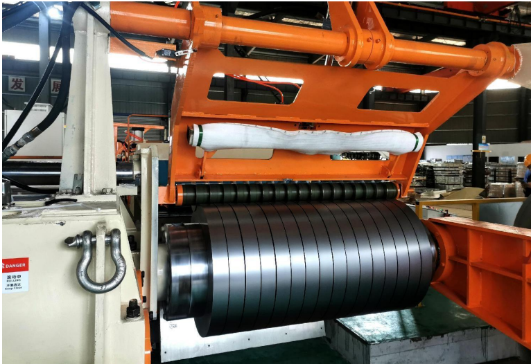
Double-blade slitting knife, saving 60% in tool change speed.
